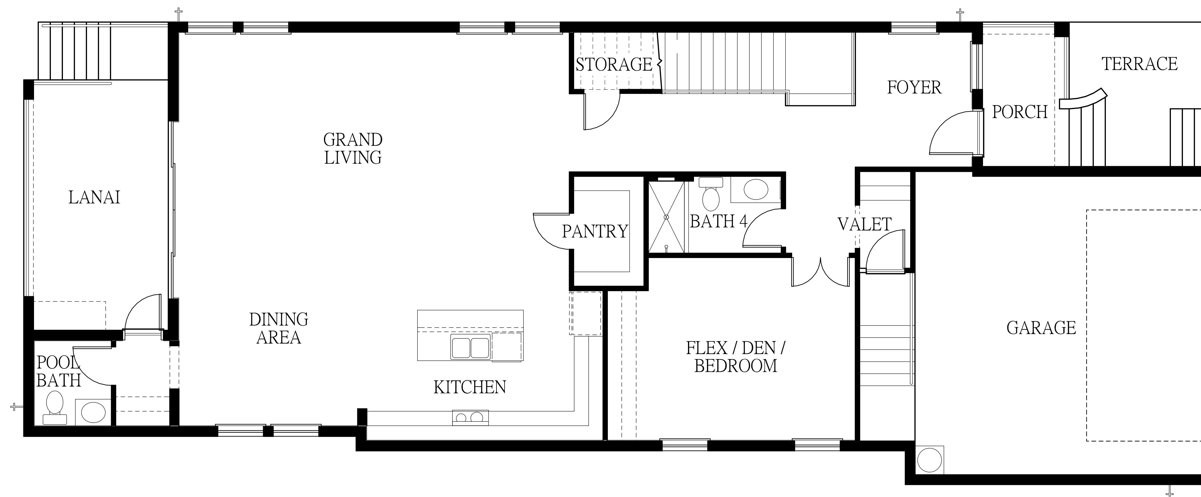
143 CHEAPEAKE FIRST FLOOR PLAN
