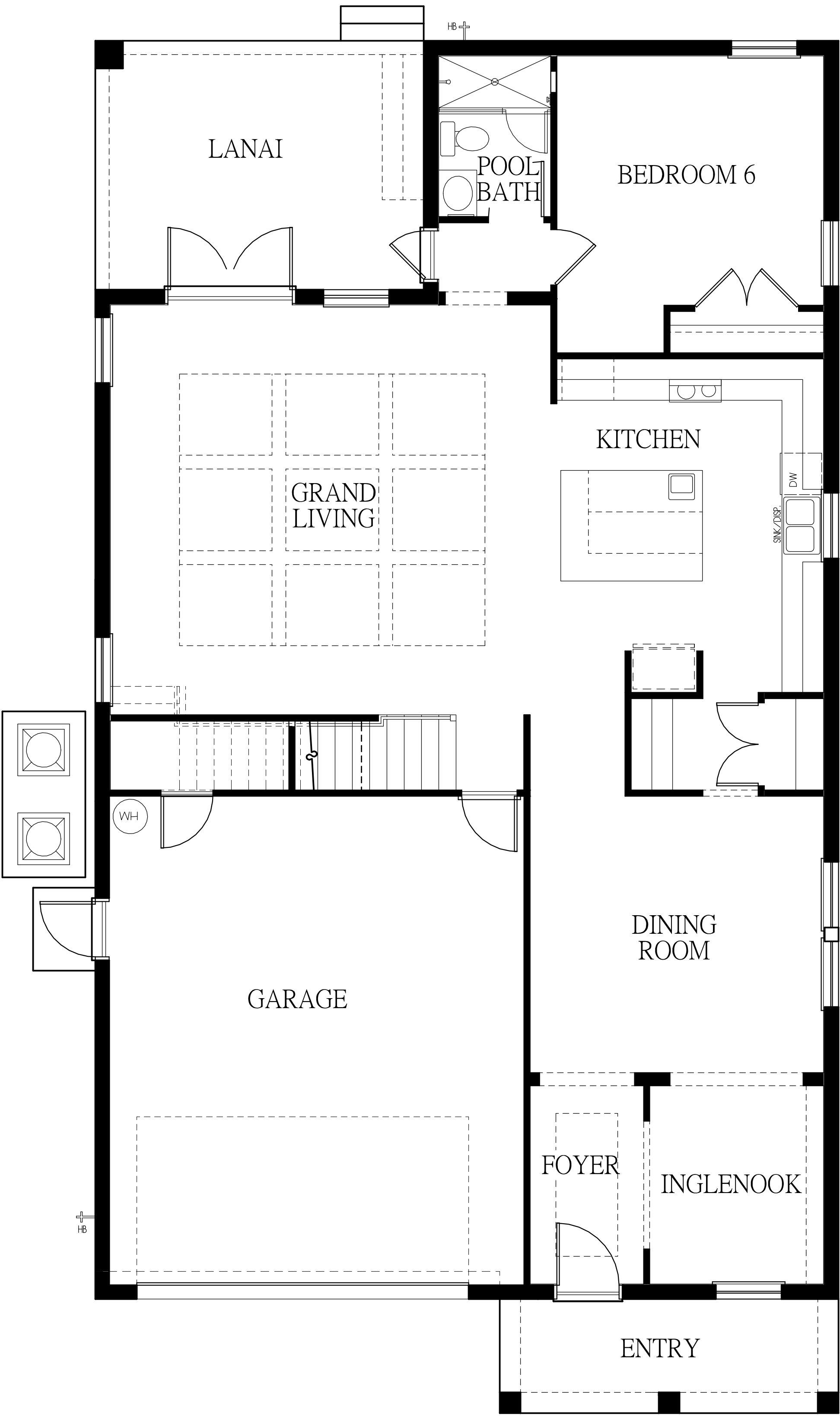
318 PARK AVE FIRST FLOOR PLAN 05-09-25
