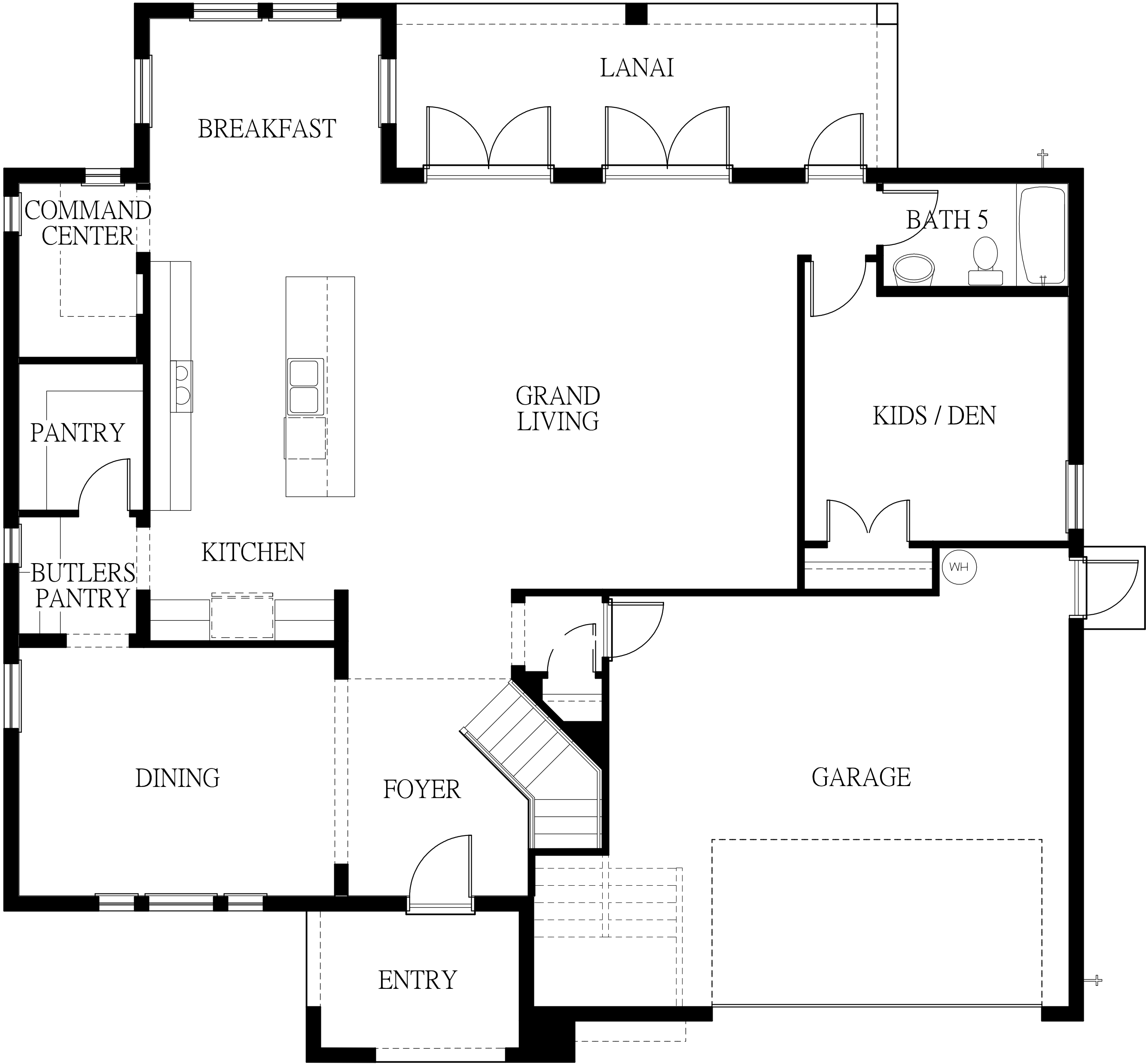
3406 PLAN FIRST FLOOR PLAN
