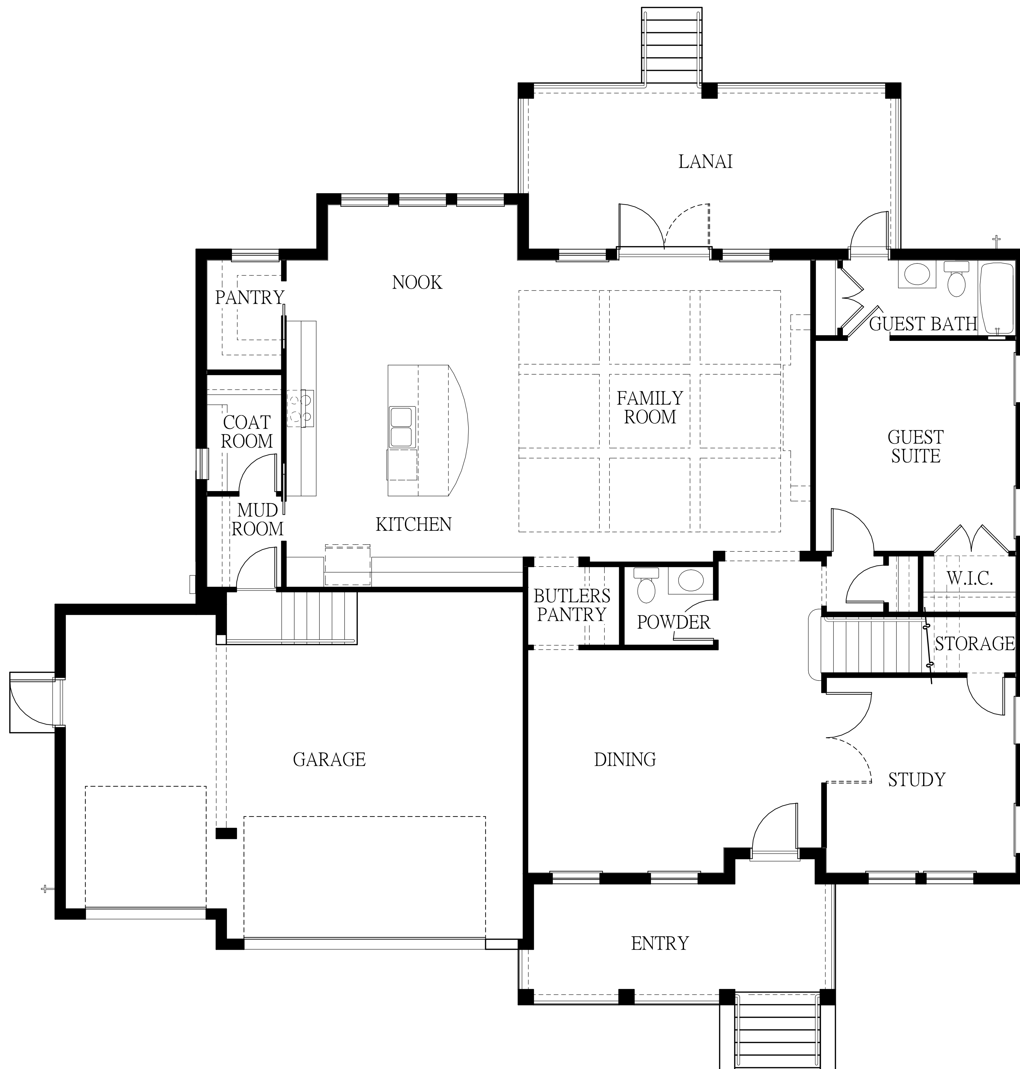
1172 SEVILLE LN N.E. FIRST FLOOR PLAN
