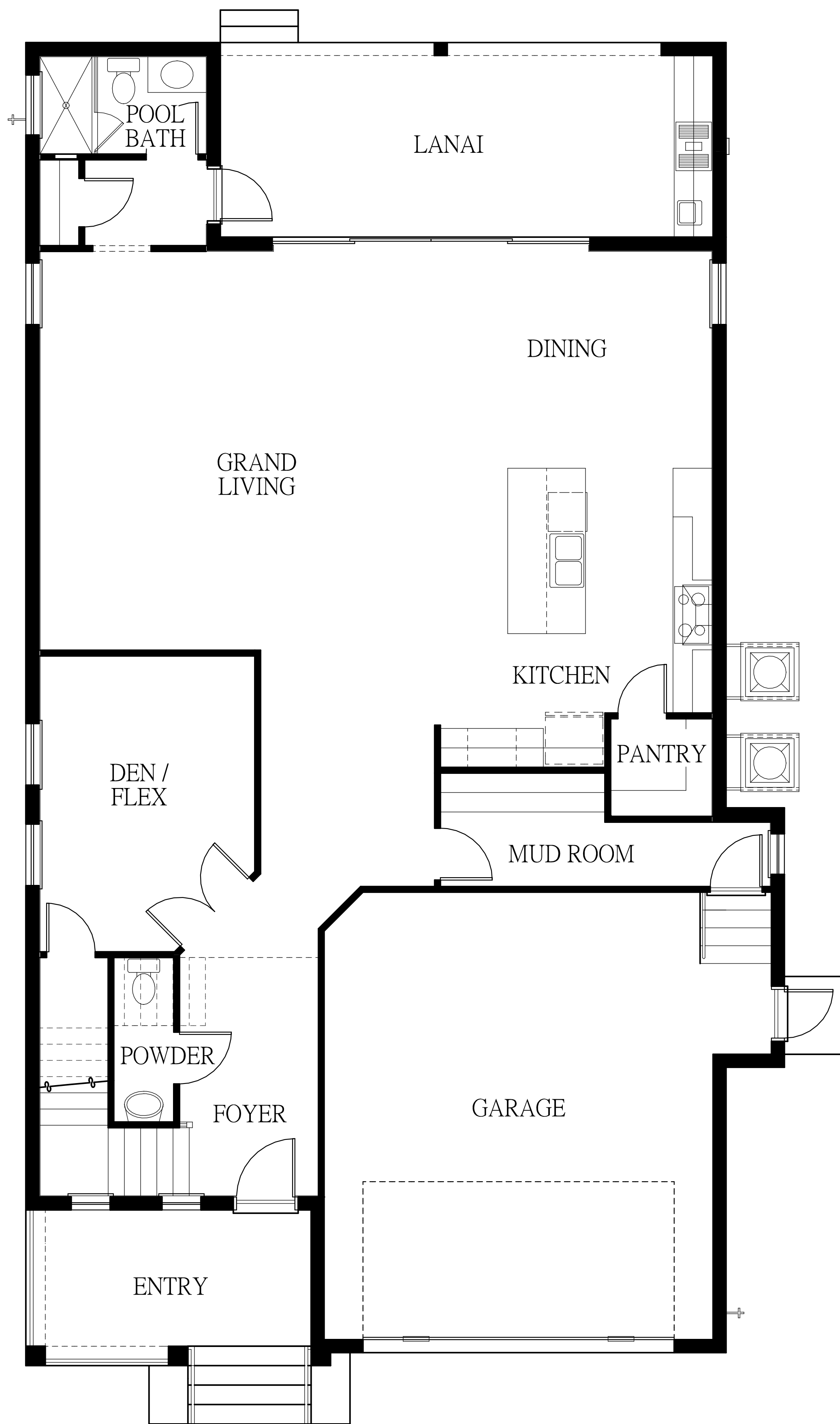
2303 N GLENWOOD DR FIRST FLOOR PLAN
