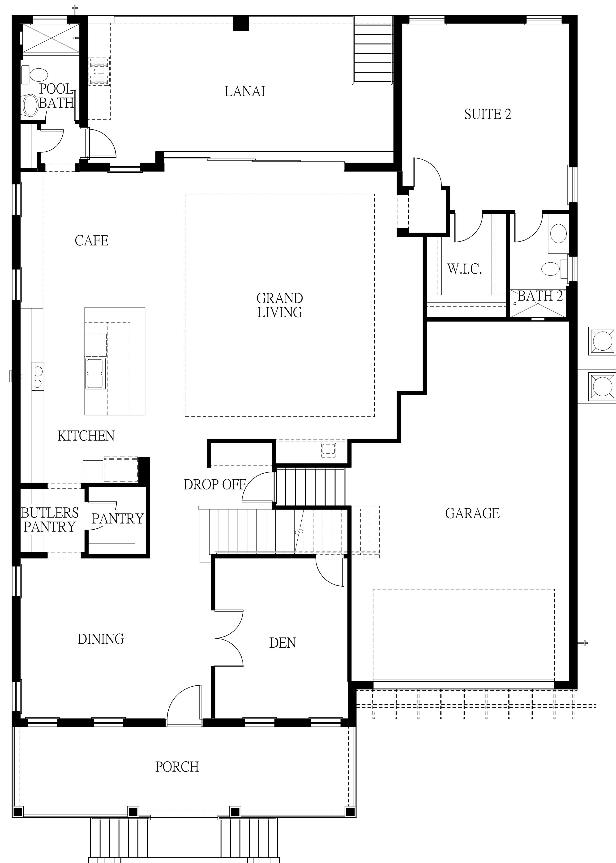
3010 KEATS FIRST FLOOR PLAN
