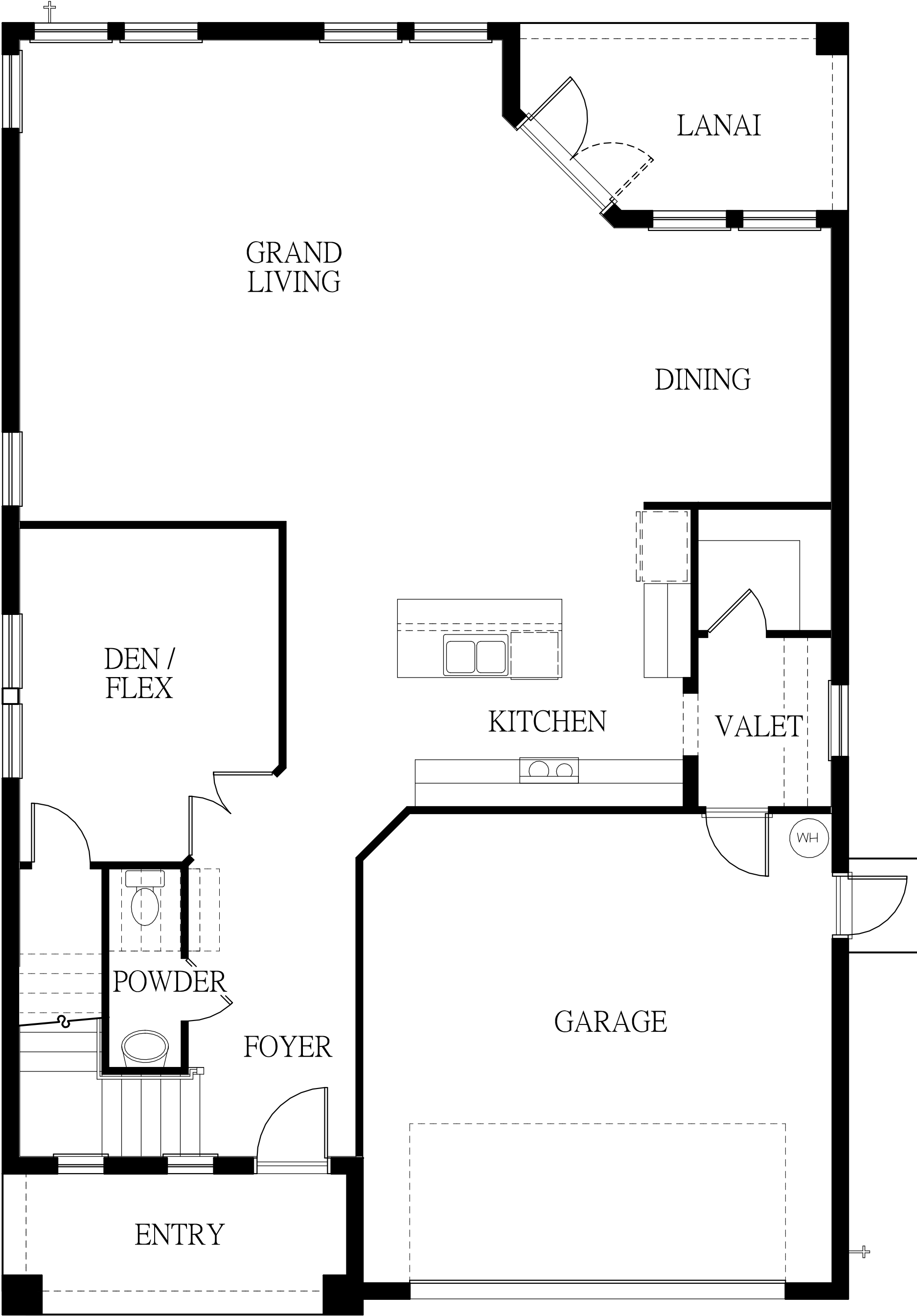
712 W. HARLAN FIRST FLOOR PLAN 09-16-26
