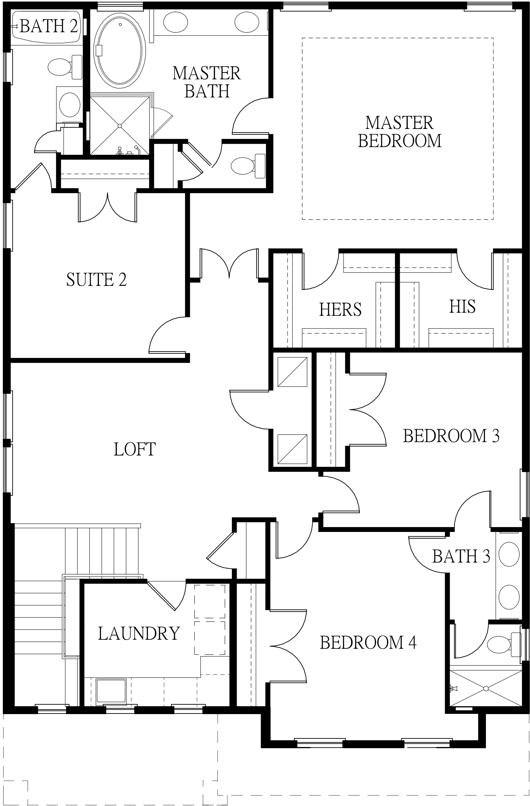
712 W. HARLAN SECOND FLOOR PLAN 09-16-26
